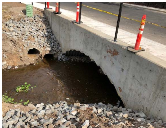
The rock slope protection for the culvert was completed.
